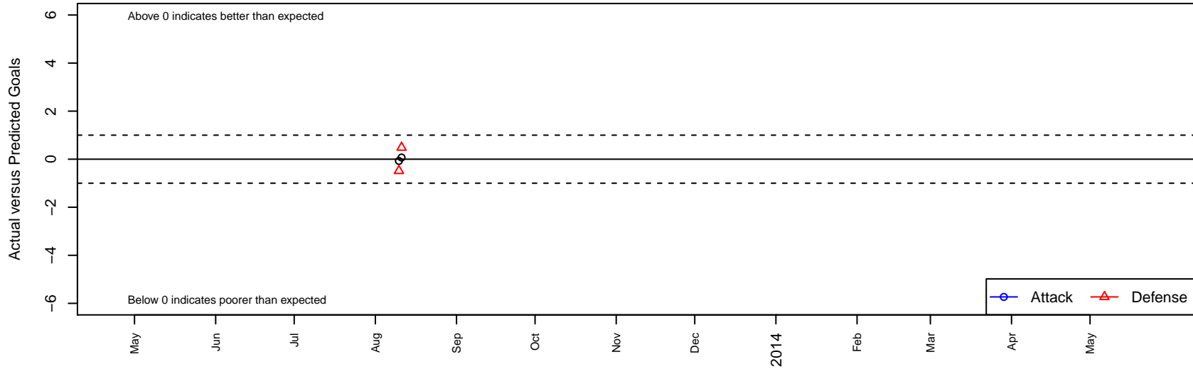
Temecula Valley SC Hawks Academy G99 Dots are actual minus expected GF (blue circles) and GA (red triangles). Blue line is smoothed change in attack strength. Red is smoothed change in defense strength.
